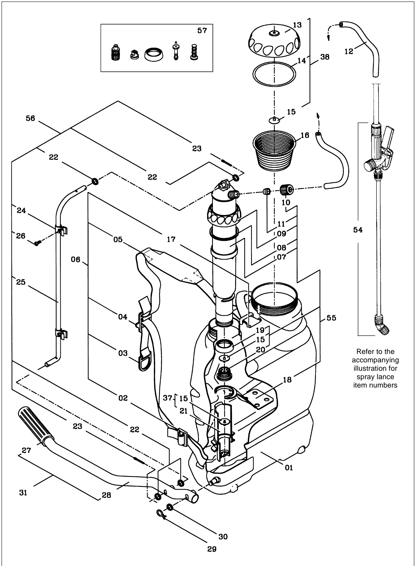
Tank Assembly
