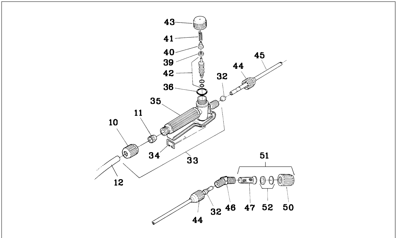
Lance Assembly
